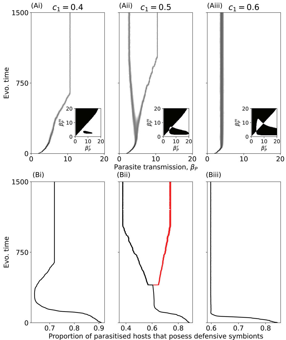
Figure 3. Parasite diversification driven by a defensive symbiont. (A) Evolutionary trajectories of parasite transmission with inset pairwise invasion plots (PIPs). Black regions in the PIPs show where the mutant can invade (where w_P(\beta_P^m | (1, \beta_P^s)) > 1 ), and white regions are where it cannot. (B) The proportion of parasitized hosts which also possess the defensive symbiont. For Bii, the red line (right branch) corresponds to the high-virulence strain, and the black line (left branch) corresponds to the low-virulence strain. Costs of host protection: (column i) c_1 = 0.4 , (column ii) c_1 = 0.5 , and (column iii) c_1 = 0.6 . These values of cost strength represent the narrow range of values with a qualitative change in evolutionary behavior. All other parameters as in Table 1.
